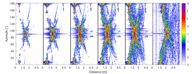
Fig. 7. The HRR profiles of a Volkswagen Golf in the elevation angle of 0^\circ using different values of \Phi and a radar measurement; from left to right: \Phi = 5^\circ, 10^\circ, 20^\circ, 60^\circ, 180^\circ , and a radar measurement. In each case, only the left side of the target is presented. From the top to the bottom of the image, the target rotates in azimuth. The range from the radar increases from left to right; each case ranging 6 meters in total. The RCS values, presented with different colors, are in \text{dB}(\text{m}^2) .
